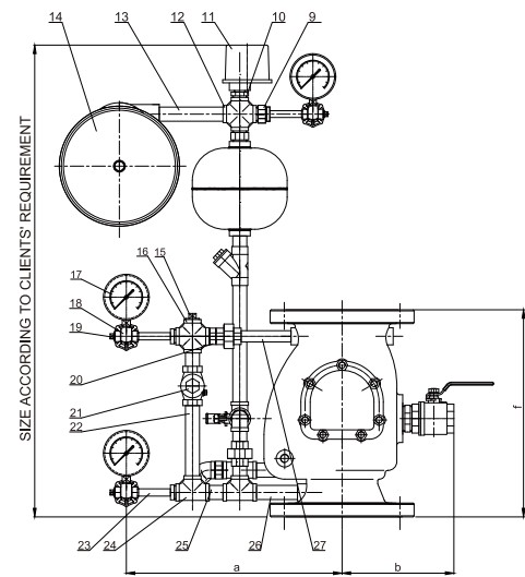
ASSEMBLY DRAWING WITHOUT COMPENSATOR SYSTEM
