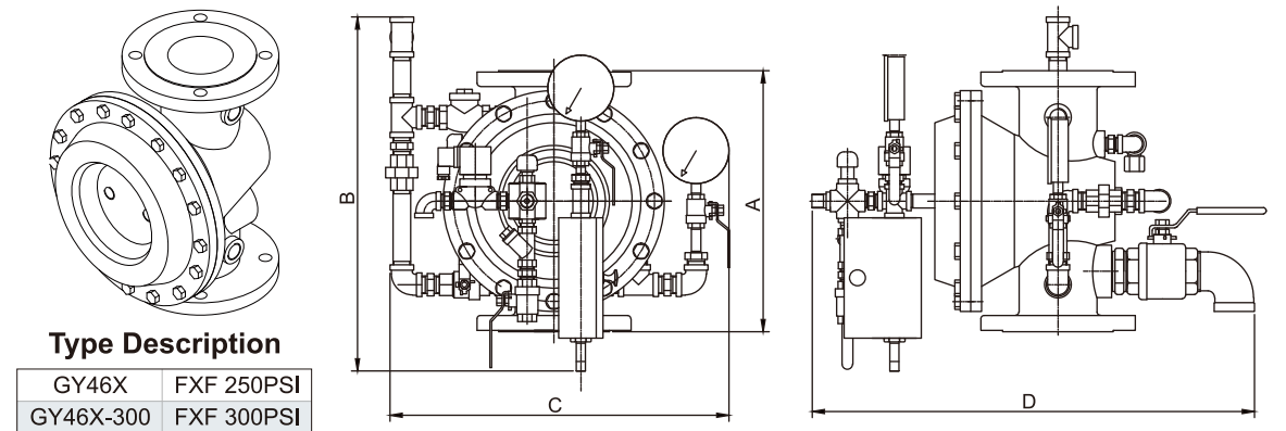
Figure 2 Outline dimensional drawing of deluge valve (Grooved * Flange connection)
