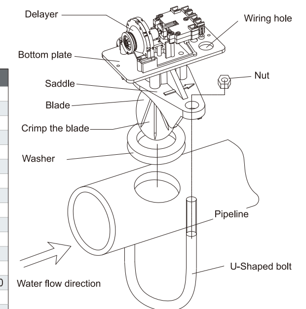
Figure 2 Installation Drawing
