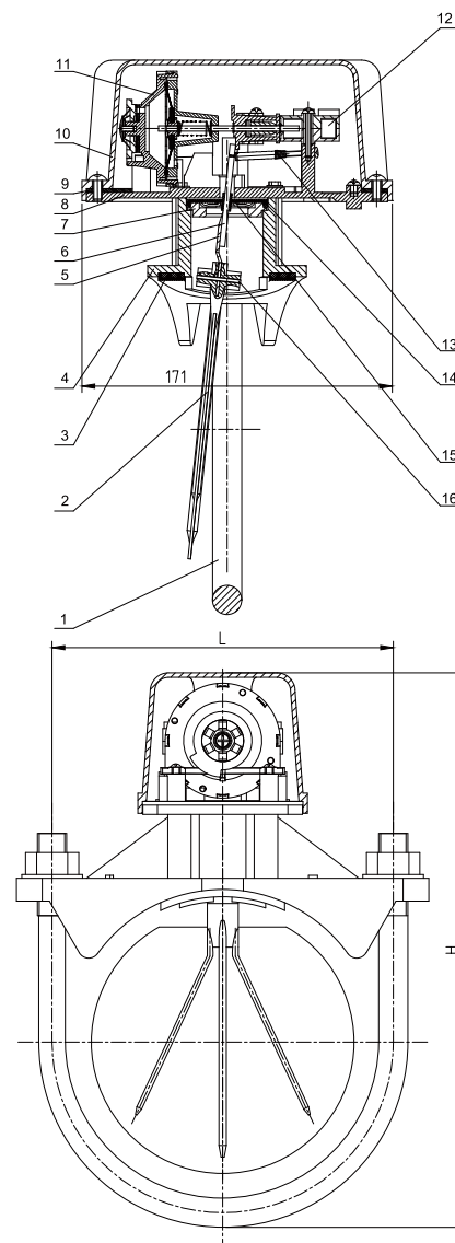
Figure 1 Outline Drawing
